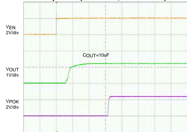
Time (50us/div)
