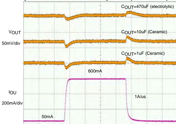
Time (100us/div)
