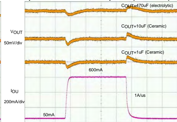
Time (100us/div)
